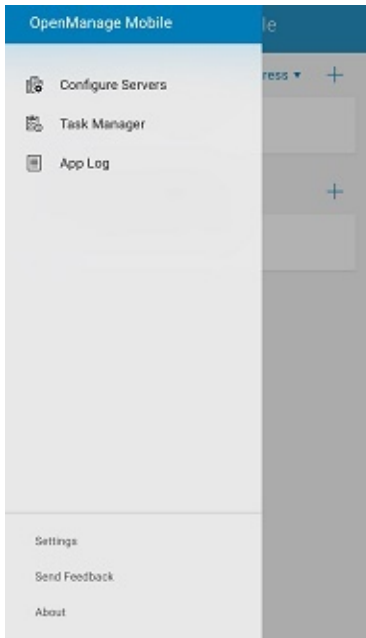
Figure 5. Navigation menu
